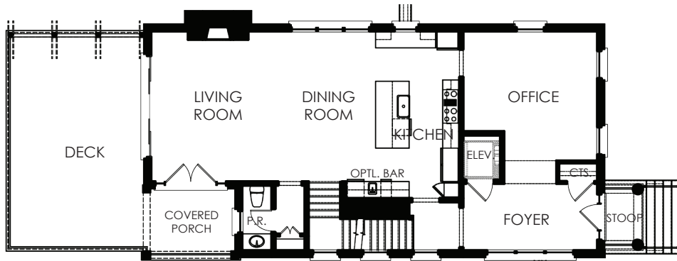
MAIN LEVEL
