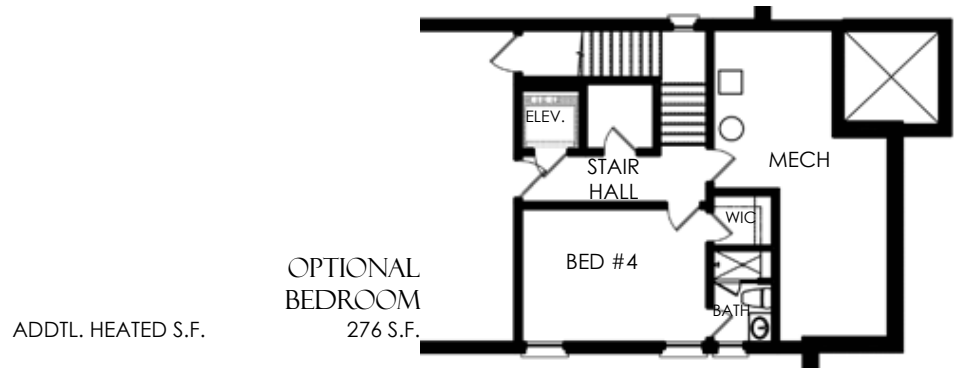
MAIN LEVEL
