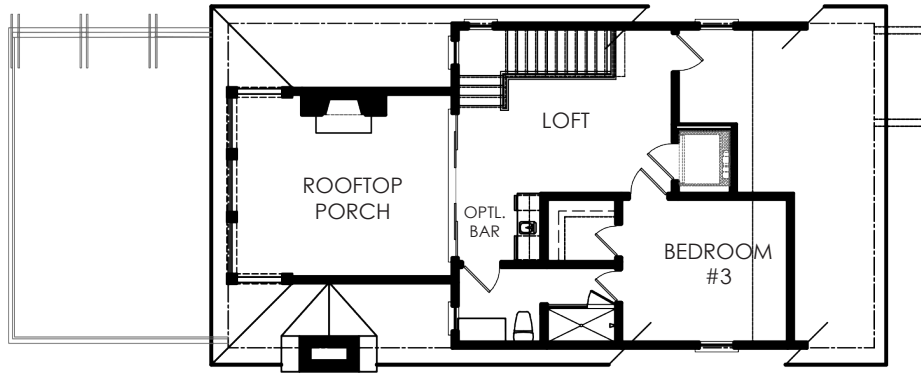
ATTIC LEVEL
